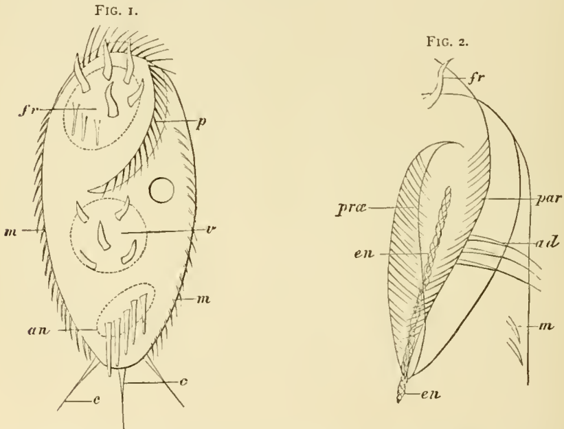
FIG. 1.—Diagrammatic outline of Stylonychia mytilus , illustrating the several ciliary systems; p , peristomal ciliary series; fr , frontal, v , ventral, an , anal styles; m , marginal, and c , caudal setæ. FIG. 2.—Peristomal ciliary system of Gastrostyla Steinii (after Sterki); ad , adoral, præ , preoral, par , paroral, and en , endoral series; fr and m , isolate elements of the frontal and marginal systems.
