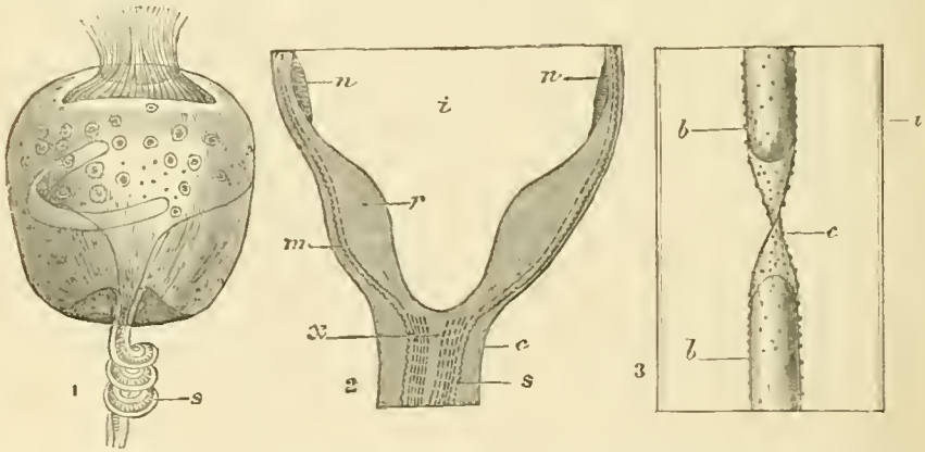
FIGS. 1 and 2. Vorticella nebulifera , Ehr. 1. Contracted zooid with s muscle-like element of the pedicle exhibiting a transversely striated aspect, \times 600 (after Everts). 2. Diagrammatic longitudinal section of lower half of the body; c , cuticle; s , central muscle-like cord of pedicle continued at m into the myophan layer of the body-wall; x , its central cavity; z , cortical layer; z , central cavity of the body; n , nucleus or endoplast, \times 1800 (after Everts).
